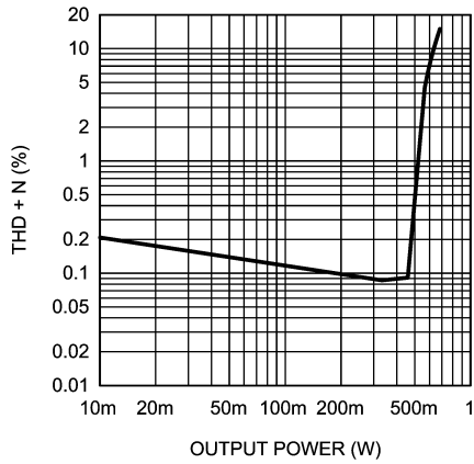
THD+N vs Power Out at V_{DD} = 3.3V , 8\Omega R_L , 1kHz, per channel
